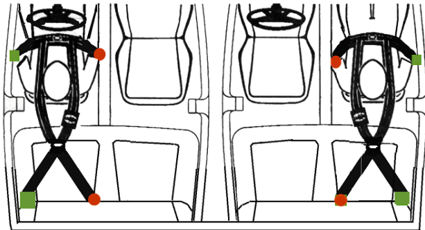
Left Side Right Side ■ Install Schroth Tail Strap w/Male End ● Factory Provided Female Receptacle
